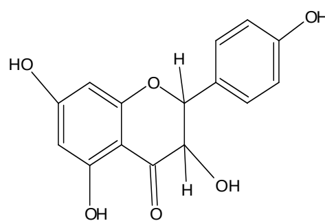
(33) Dihydrokaempferol
