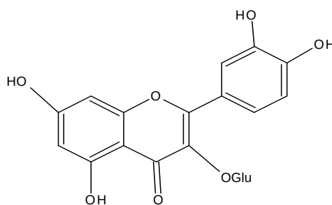
(37) 3-O-glucosyl Quercétin
