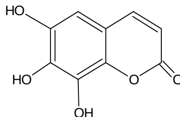
(13) 6,7,8-trihydroxycoumarine
